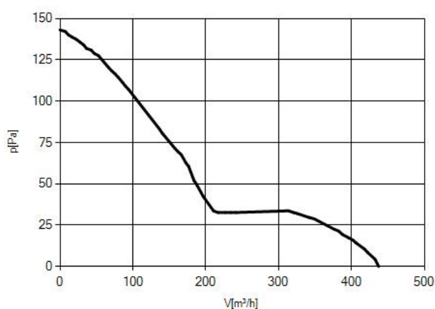
Air performance
